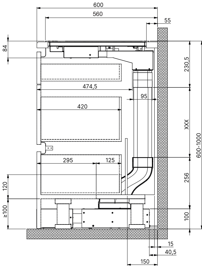
Installation for recirculation with grille for skirting board
