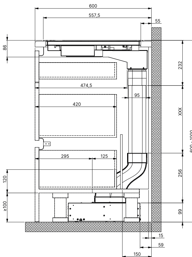
Installation for lateral exhaust air system
